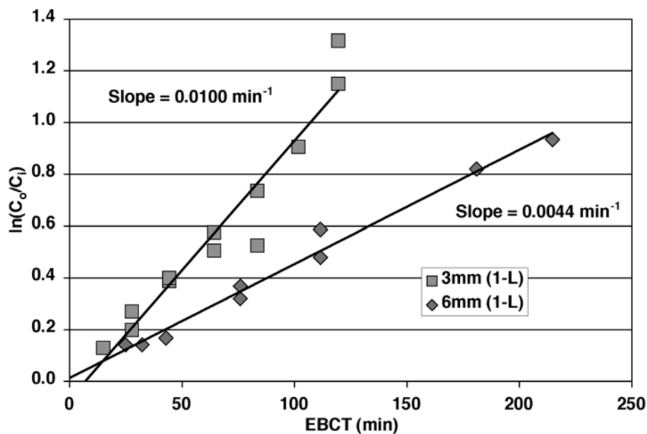
Fig. 4. \ln(C_0/C_1) vs EBCT for 1-L TBR experiments with two different size supports. The liquid recirculation rate was 200 mL/min. The slopes of the regression line provide an estimate of the overall mass transfer coefficient in the system. The intercepts are not significantly different from zero at the 95% confidence level.
